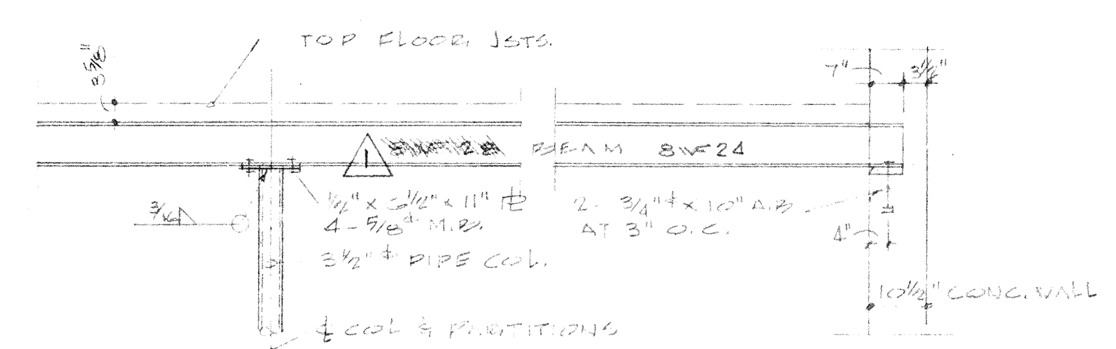
DETAIL A 1/2" = 1'-0"
