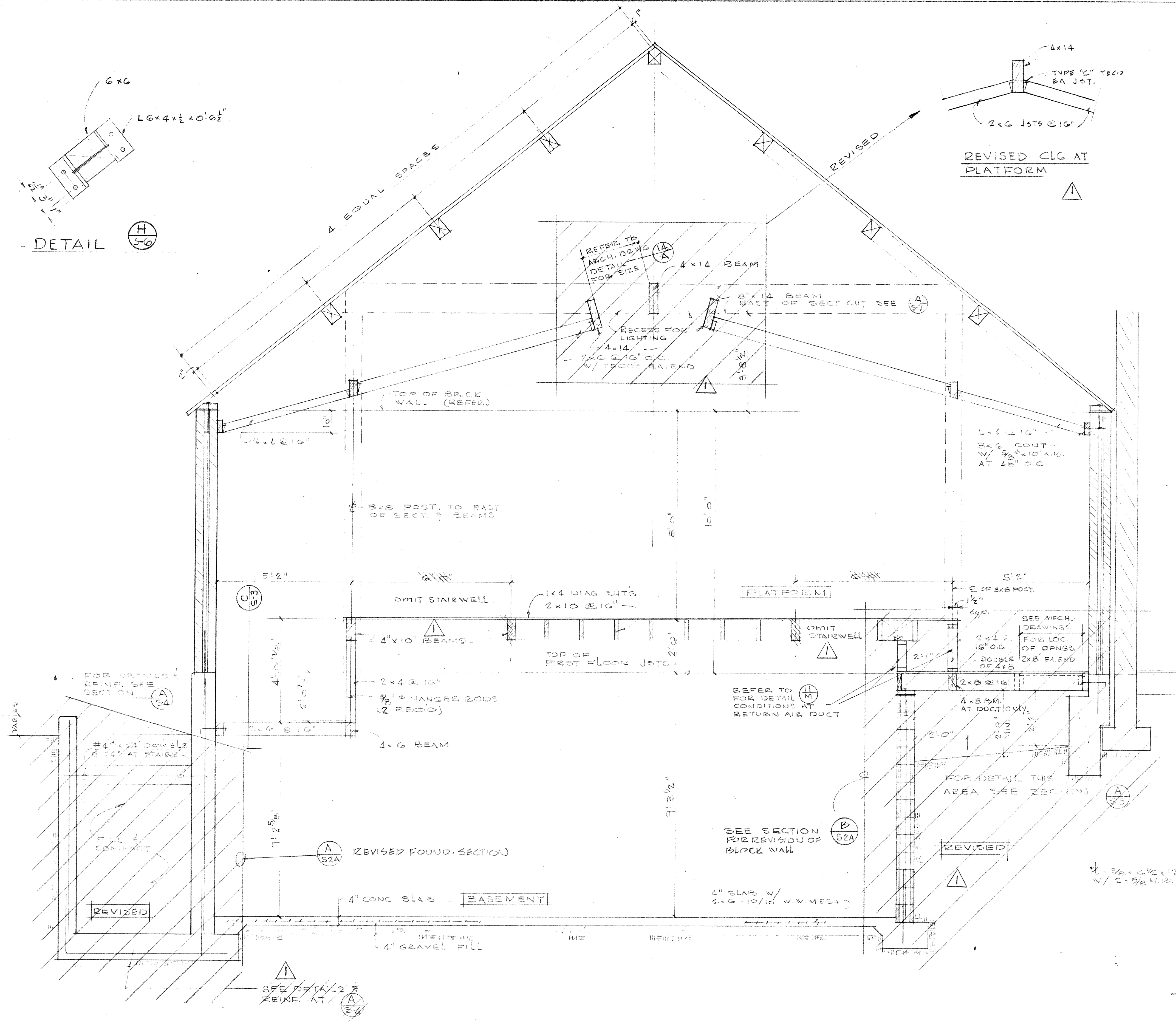
SECTION A 1/2" = 1'-0"
