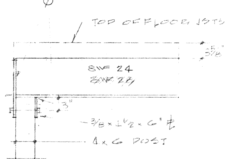
DETAIL A 1/2" = 1'-0"
