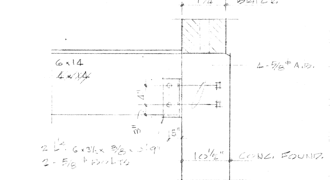
DETAIL G 1" = 1'-0"
